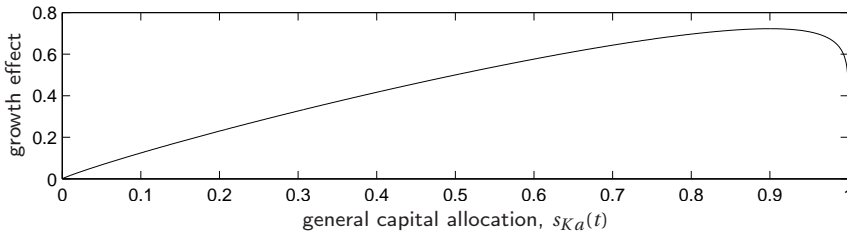
Figure 6.3: Growth effect of investment in general capital. The production coefficient is \alpha = .9 .
