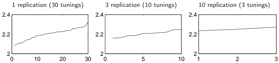
Figure 2.12: Distribution of the performance after tuning. The y-axis shows the average performance after tuning. The x-axis shows how many REVC runs resulted in an average performance of that level or lower. Note that the median is similar in each graph.
