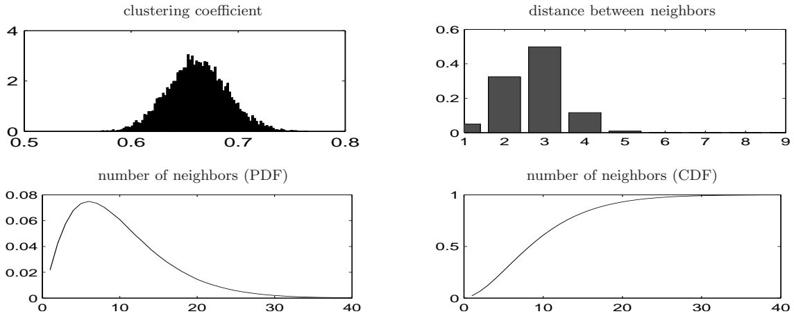
Figure 2: Network statistics. The two upper graphs are normalized histograms.
