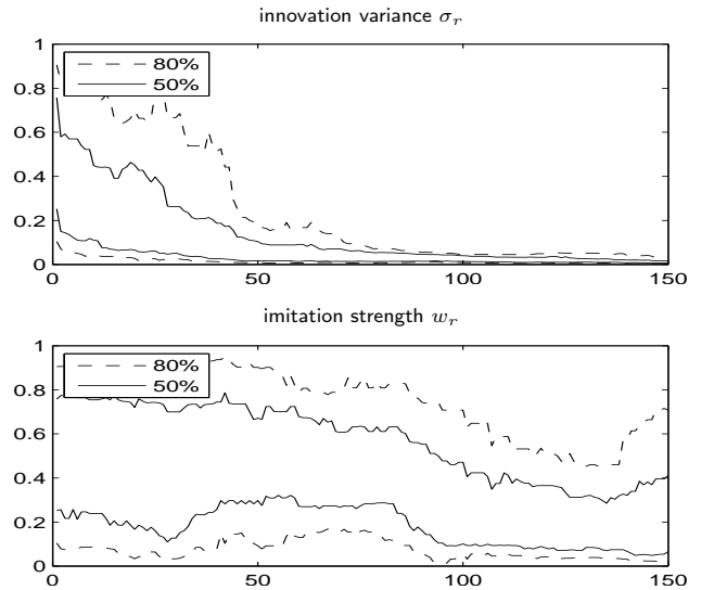
Figure 2: Example of how the density of \mathcal{B}_i changes during the search. The x -axis shows the iterations i of the search, the y -axis shows the parameter ranges. Each point i along the x -axis is a crosscut through the corresponding calibration \mathcal{C}_i , reflecting the density of the 100 best settings \mathcal{B}_i along the parameter. 50% of \mathcal{B}_i are concentrated between the two solid lines, 80% between the dashed lines. The graphs are taken from an experiment with 200 agents, 2 nonviable technologies and low vulnerability.
